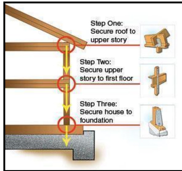
Figure 4: Continuous Load Path
