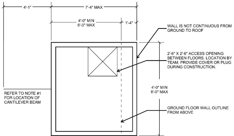
SECOND FLOOR LEVEL PLAN
