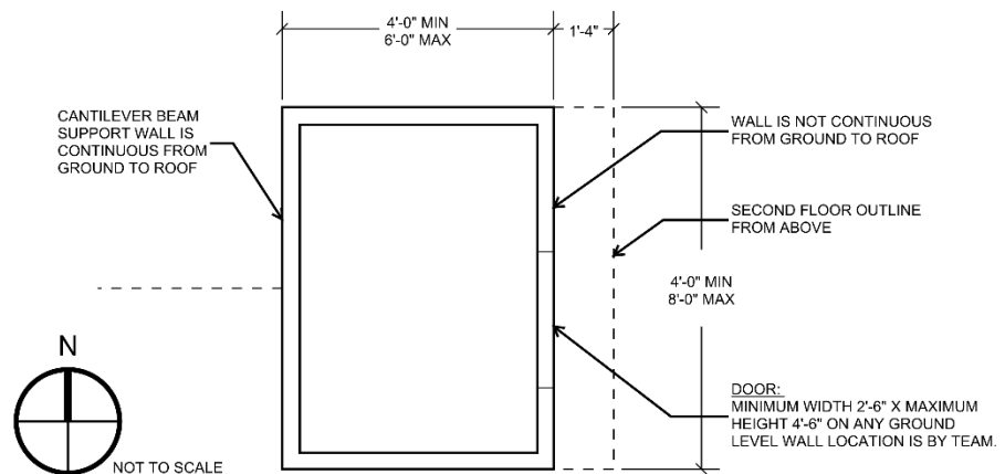
GROUND FLOOR LEVEL PLAN
