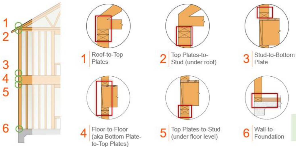
Figure 5: Continuous Load Path Resisting Uplift Forces
