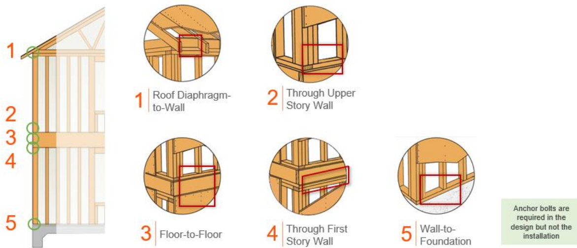
Figure 6: Continuous Load Path Resisting In-Plane Forces
