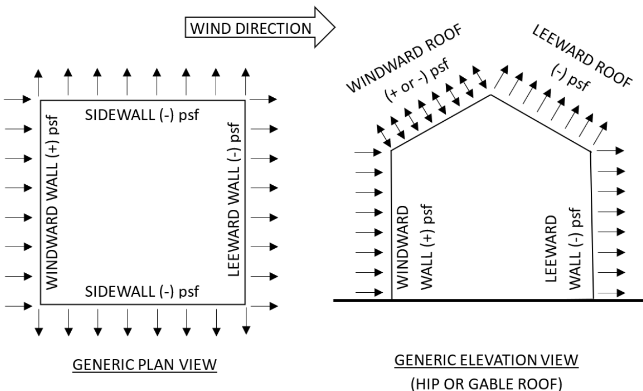
Figure 3: Wind Pressure Diagram
