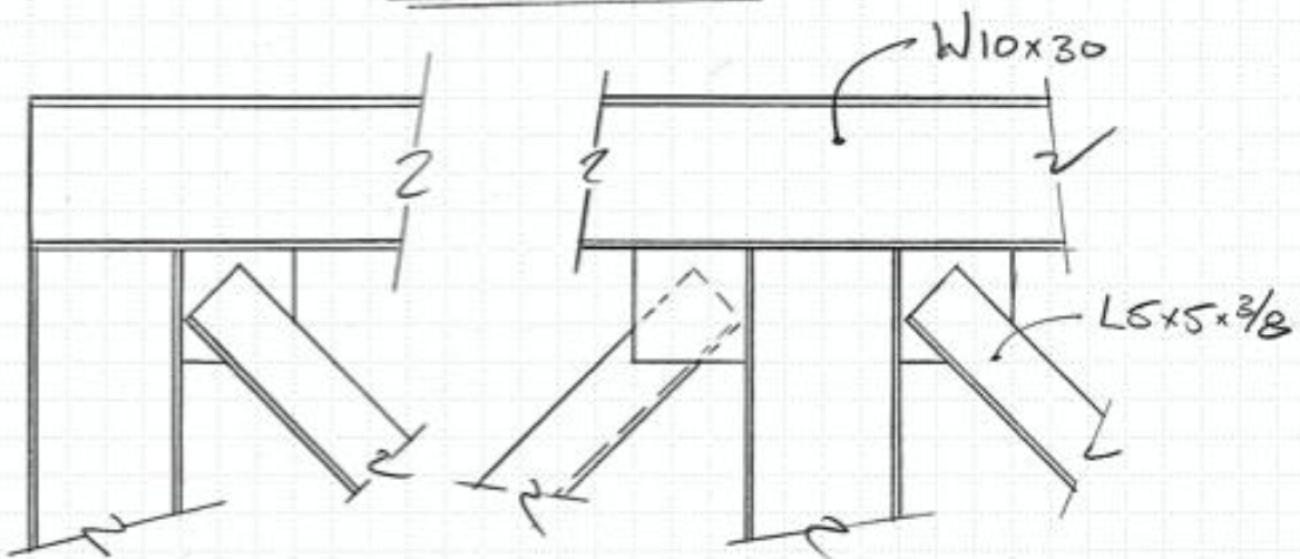
CONNECTION SCHEMATICS
